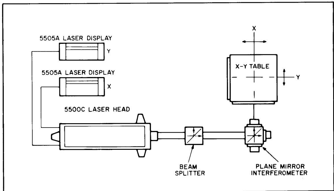
Figure 6. Autoreflection Alignment
