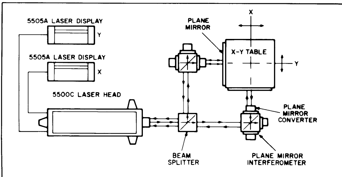
Figure 4. Dual Axis Measurement
