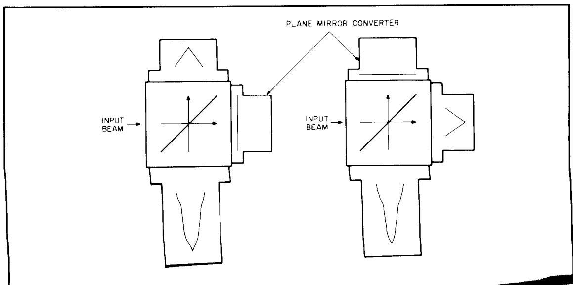
Figure 2. Retroreflector and Plane Mirror Mounting
