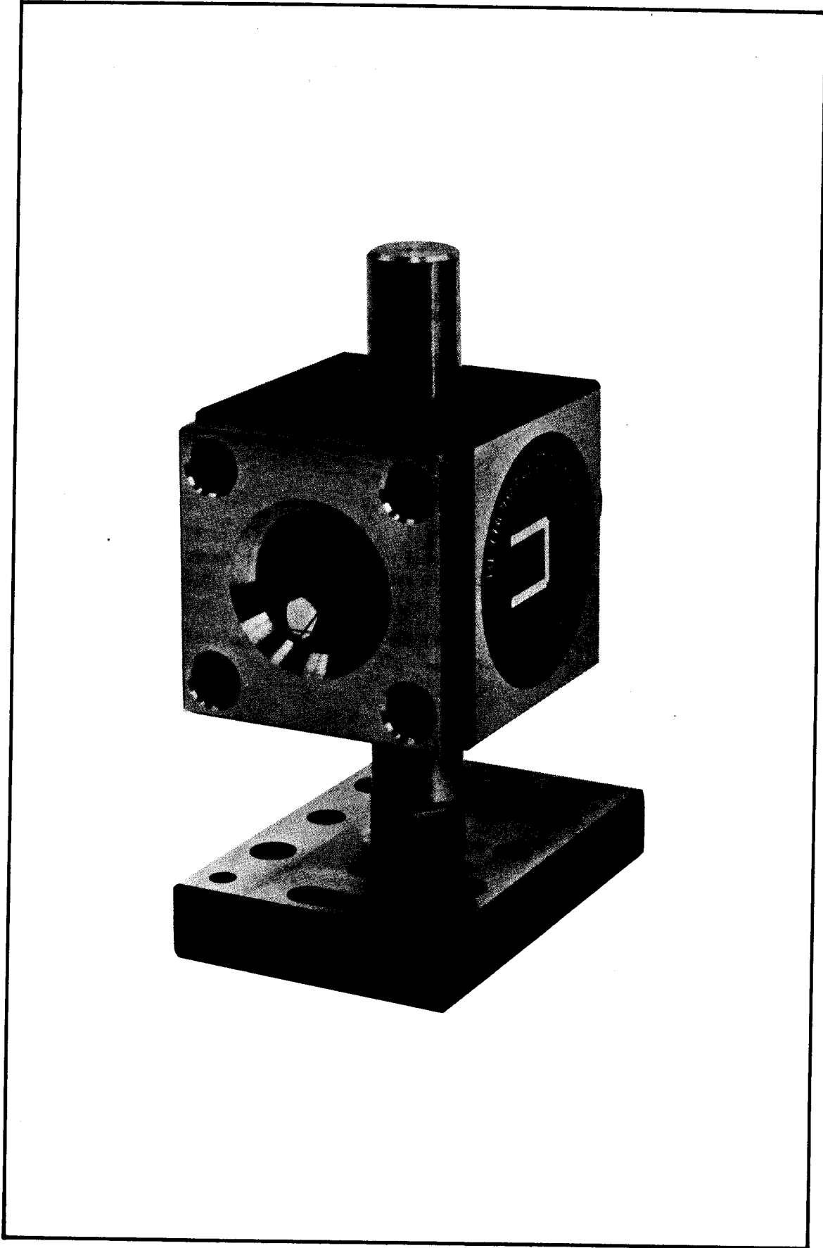
Figure 1. 10550B Laser Reflector, Mount and Stand
